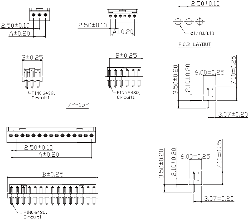
PartNo.: 2504S-XXTR-L
